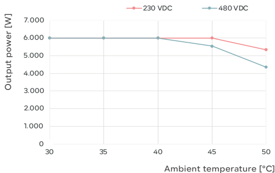
Fronius Primo GEN24 6.0 208-240 [Plus] Temperature derating (240VAC)
